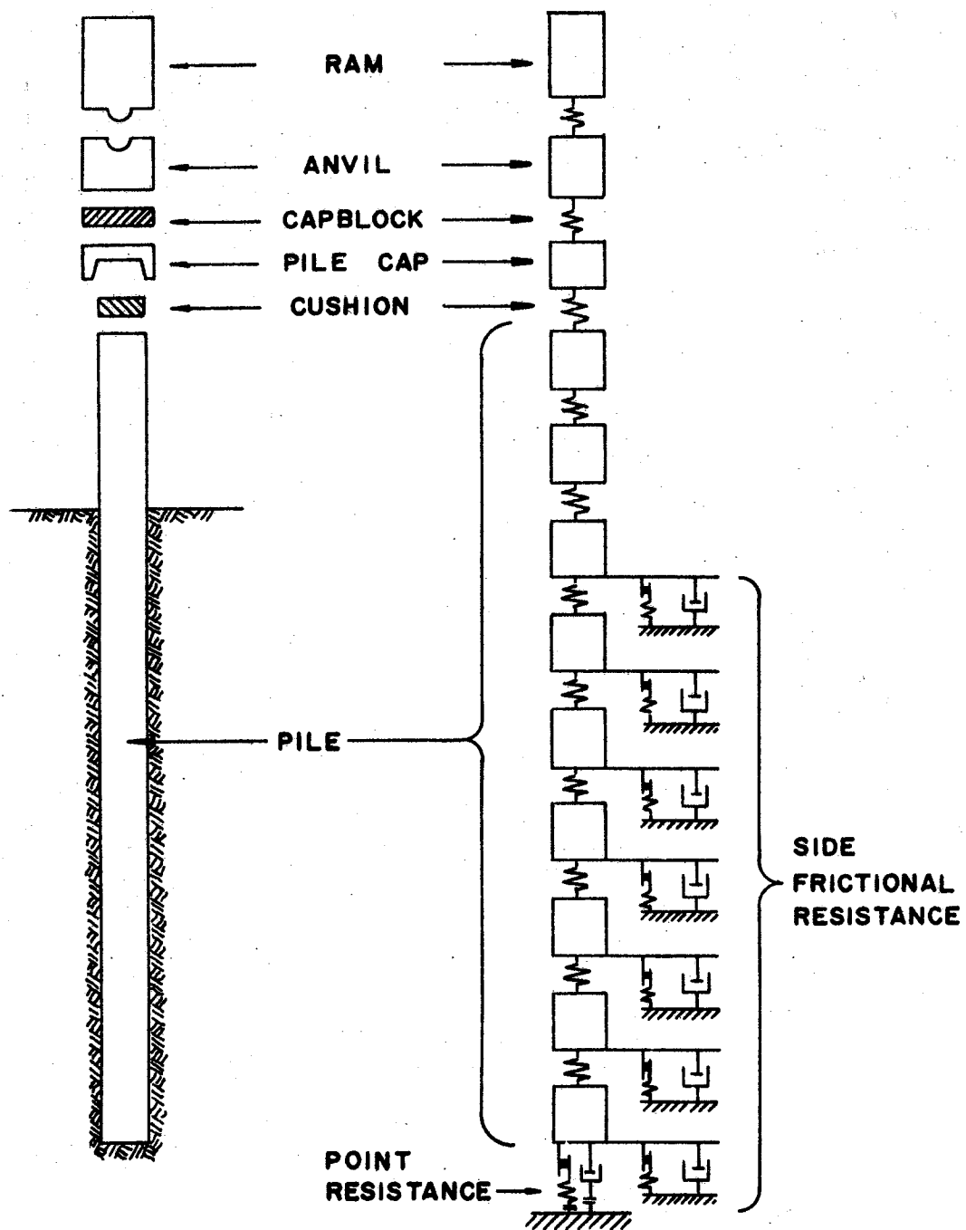
(B) IDEALIZED SYSTEM
