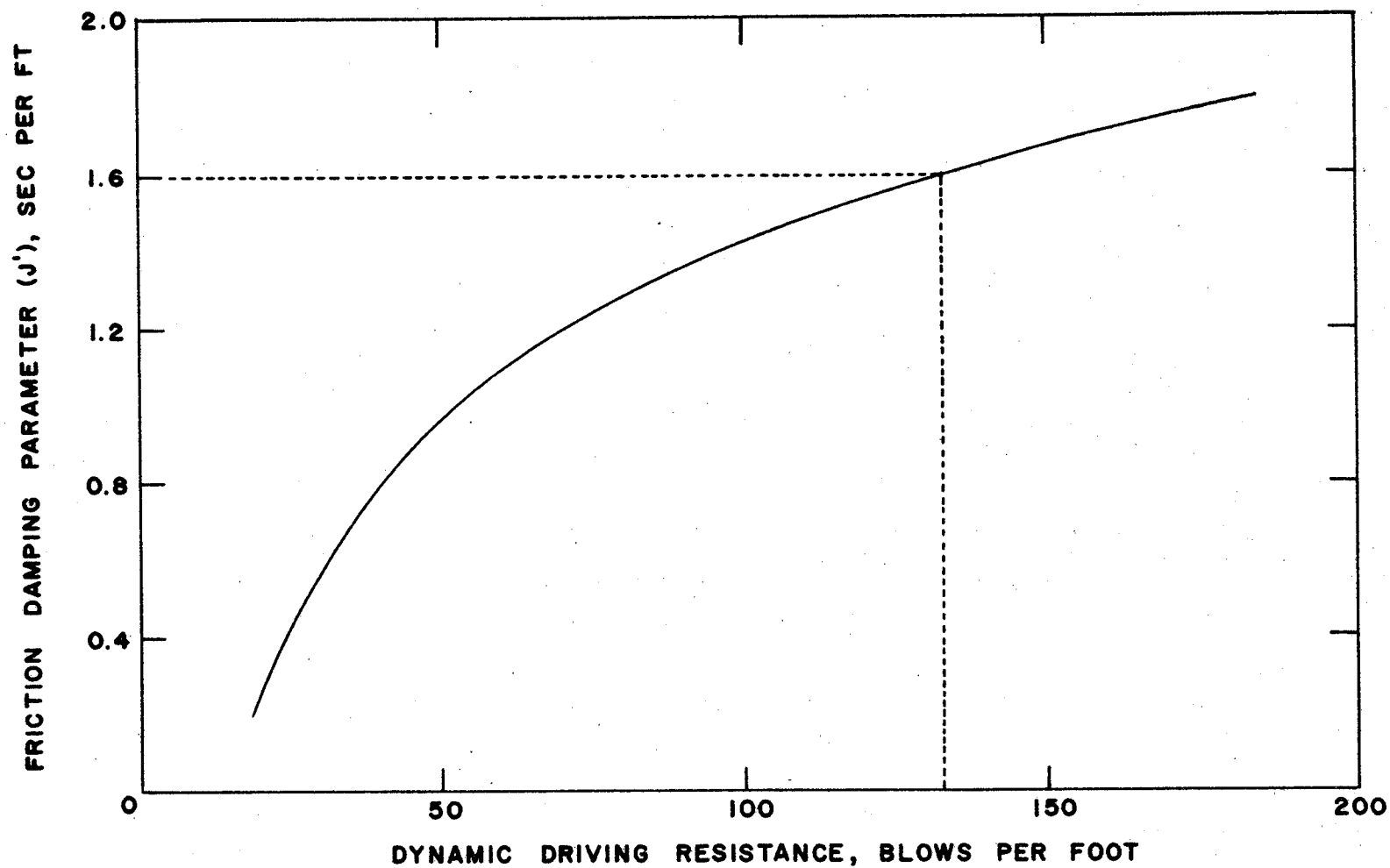
FIGURE 18 - FRICTION DAMPING PARAMETER VERSUS DRIVING RESISTANCE FOR BELLEVILLE LOAD TEST PILE NO. 1
