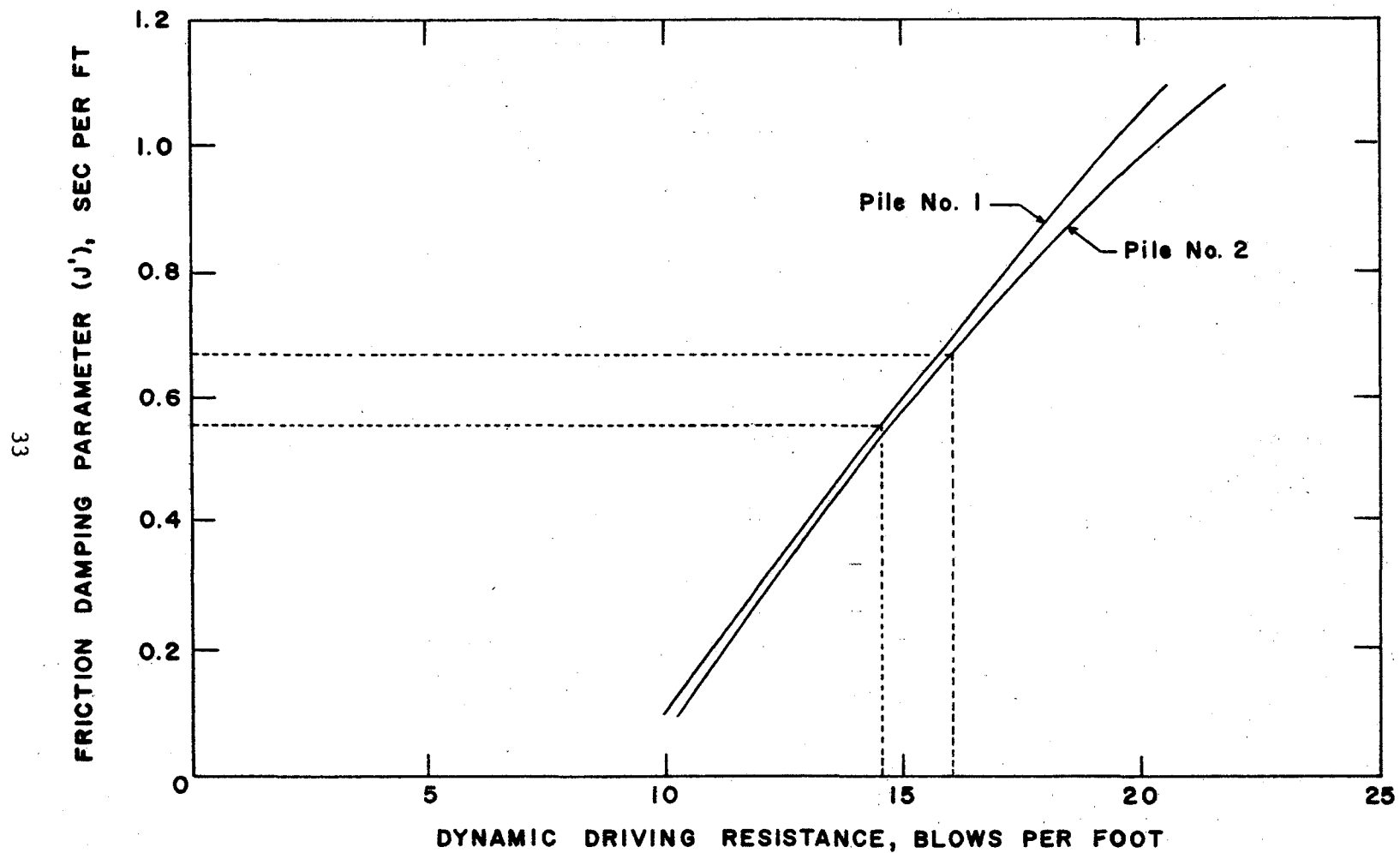
FIGURE 12 - FRICTION DAMPING PARAMETER VERSUS DRIVING RESISTANCE FOR PORT ARTHUR PILES
