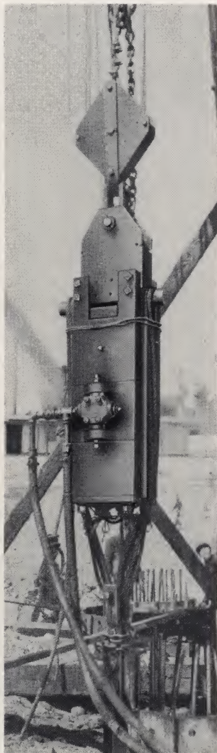
Pulling piles with inverted McKiernan-Terry Double-Acting Pile Hammers. Left —No. 6 Hammer pulling 14-inch arch web steel piling, using standard rig shown at right of page. Center —Pulling sheet piling 44 feet long, concreted to a depth of 41 feet—without difficulty. Right —Special pulling rig, used in England, made of steel bars with grips to pile webs.
