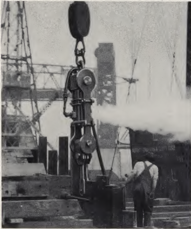
(Above) New York City. McKiernan-Terry No. E-4 Double-Acting Pile Extractor removing steel sheet piling used in the construction of the East River Drive. Contractor, Merritt-Chapman & Scott Corp.
