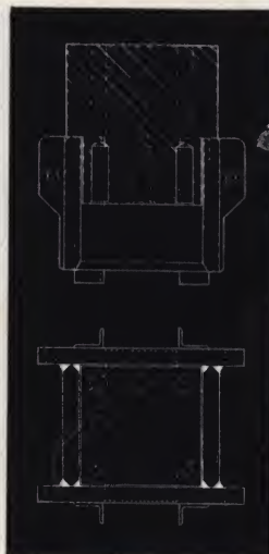
No. A-1944. For concrete piles with extended reinforcing rods.
