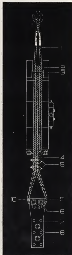
Cable pulling rig commonly in use. Can be furnished for Nos. 5, 6 and 7 McKiernan-Terry Double-Acting Pile Hammers.
