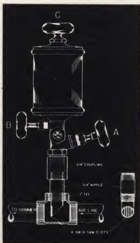
Air lubricator
