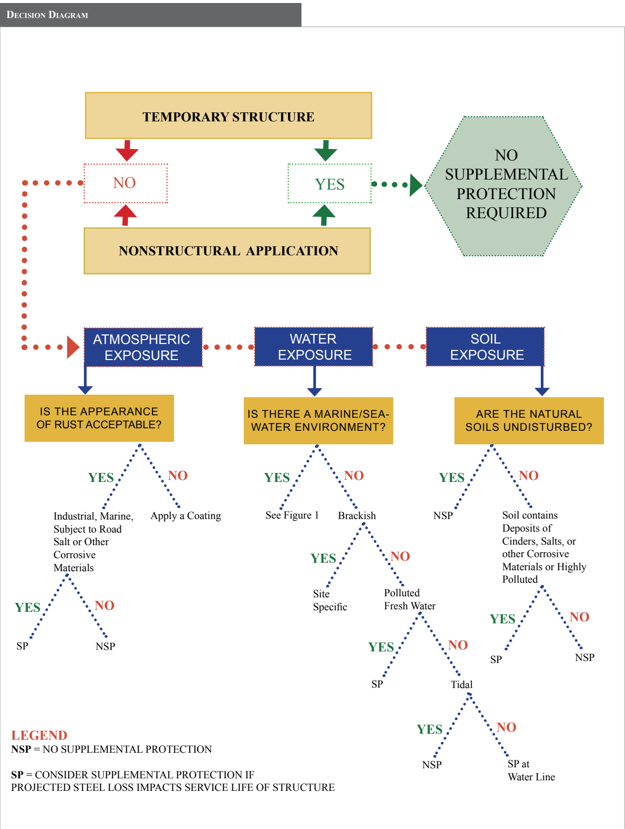
FIGURE 2. CORROSION PROTECTION CONSIDERATIONS
