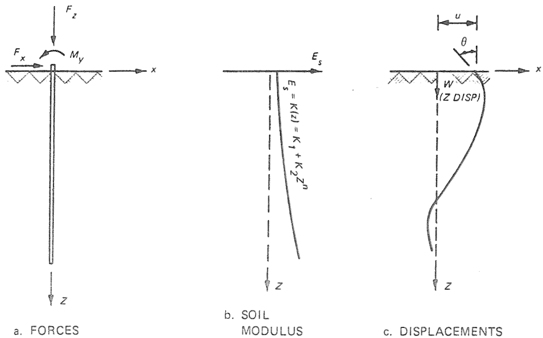
Figure A1. Notation for laterally loaded piles
