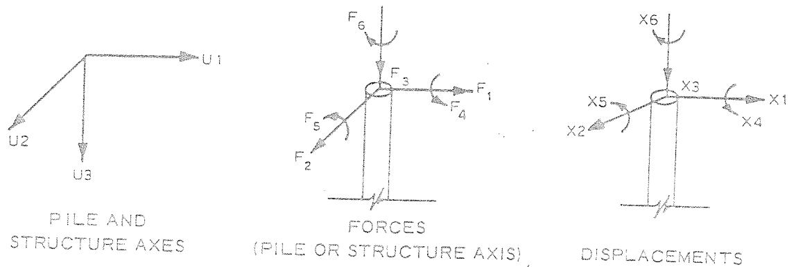
Figure 1. Coordinate system for three-dimensional system
