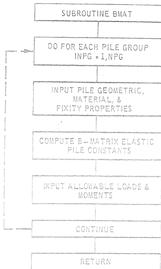
Figure 5. Flow chart of sub- routine BMAT for LMVDPIL
