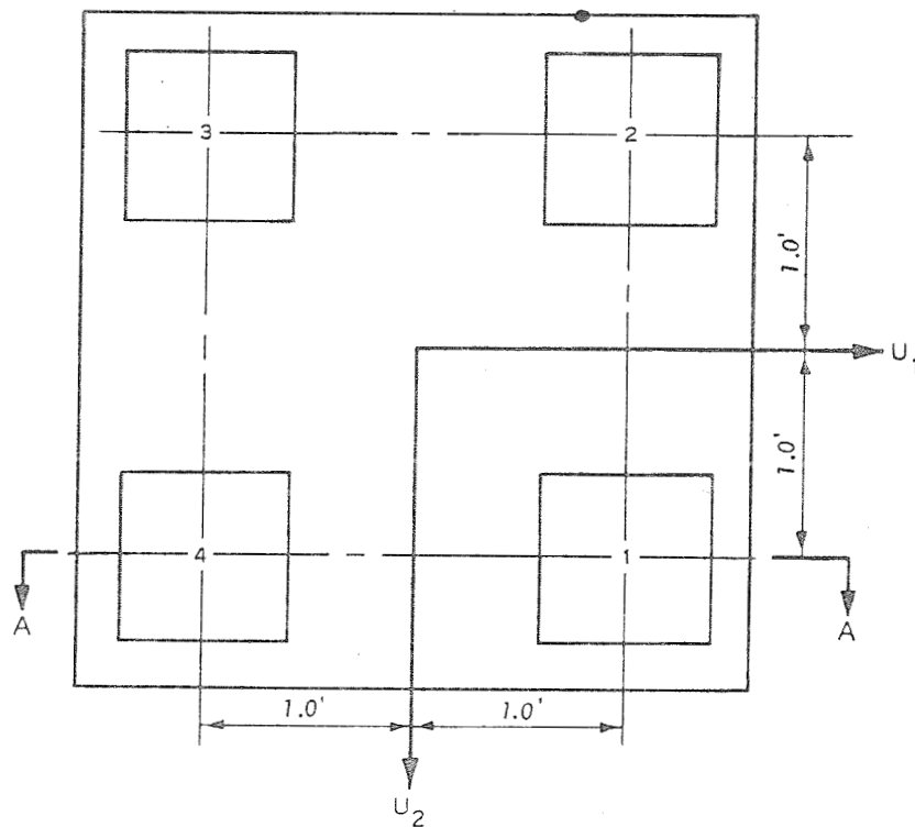
Figure 16. Plan view of example problem 7
