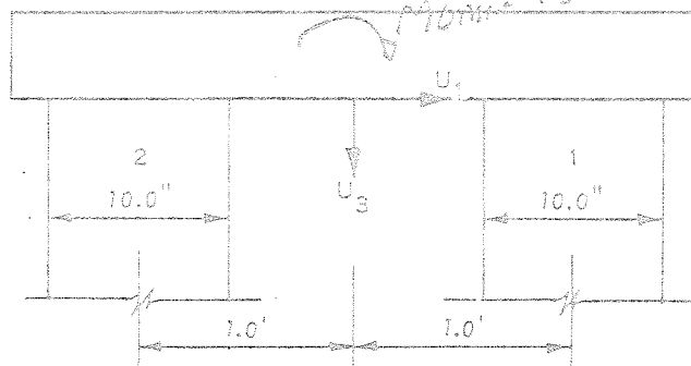
Figure 6. Physical problem for example problem 1
