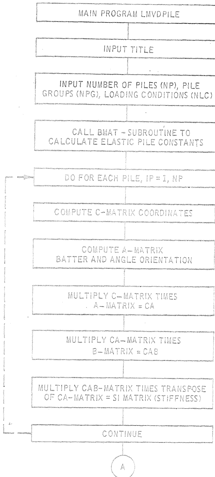
Figure 4. Flow chart for LMVDPILE (sheet 1 of 2)
