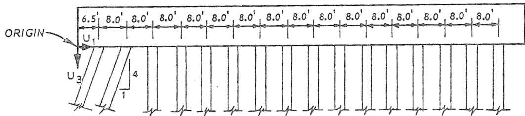
Figure 14. Physical problem for example problem 6
