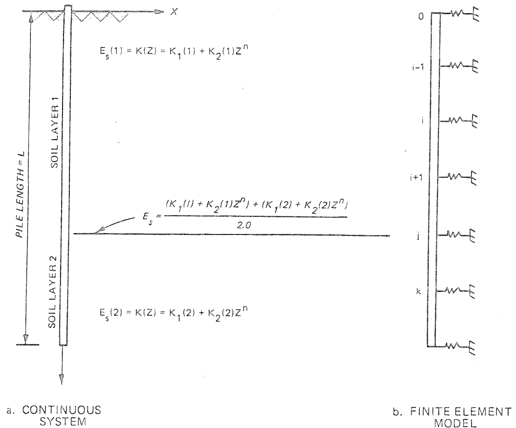
Figure A4. Finite element model of pile-multilayered soil system
