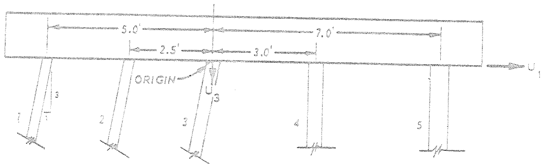
Figure 10. Physical problem for examples 3, 4, and 5
