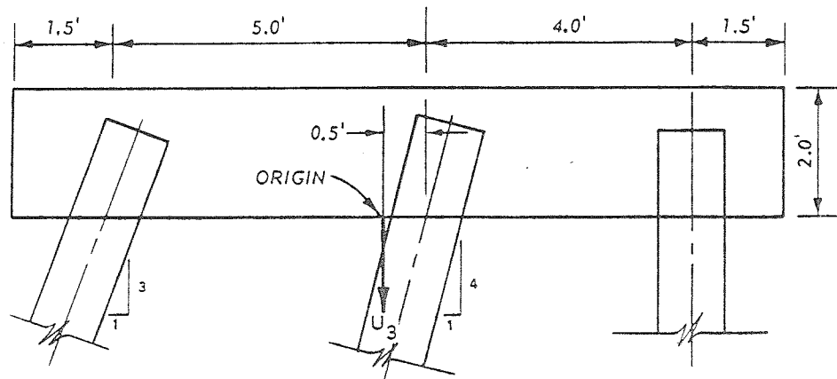
Figure 24. Section A-A for example problem 10
