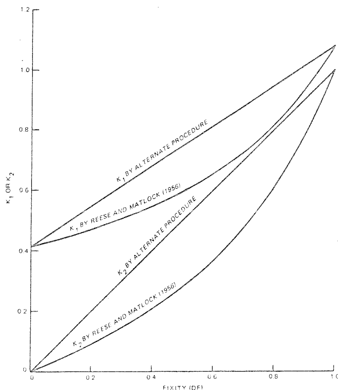
Figure A2. Comparison of stiffness coefficients
