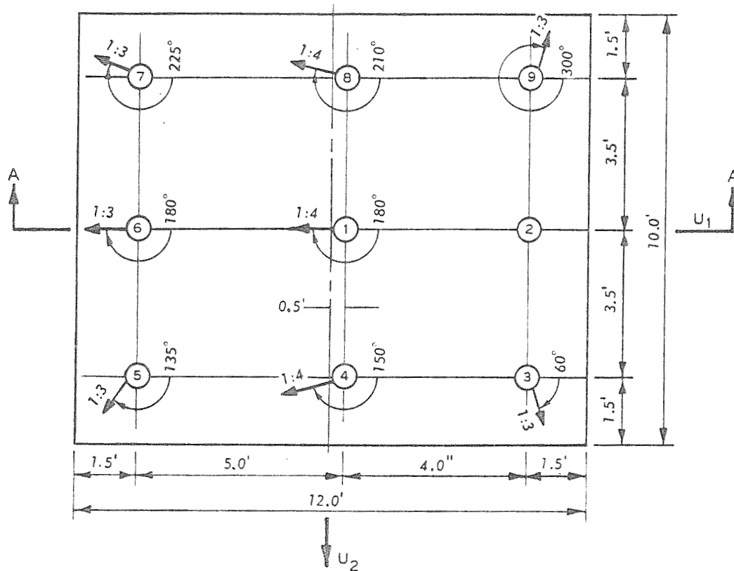
Figure 23. Plan view of example problem 10
