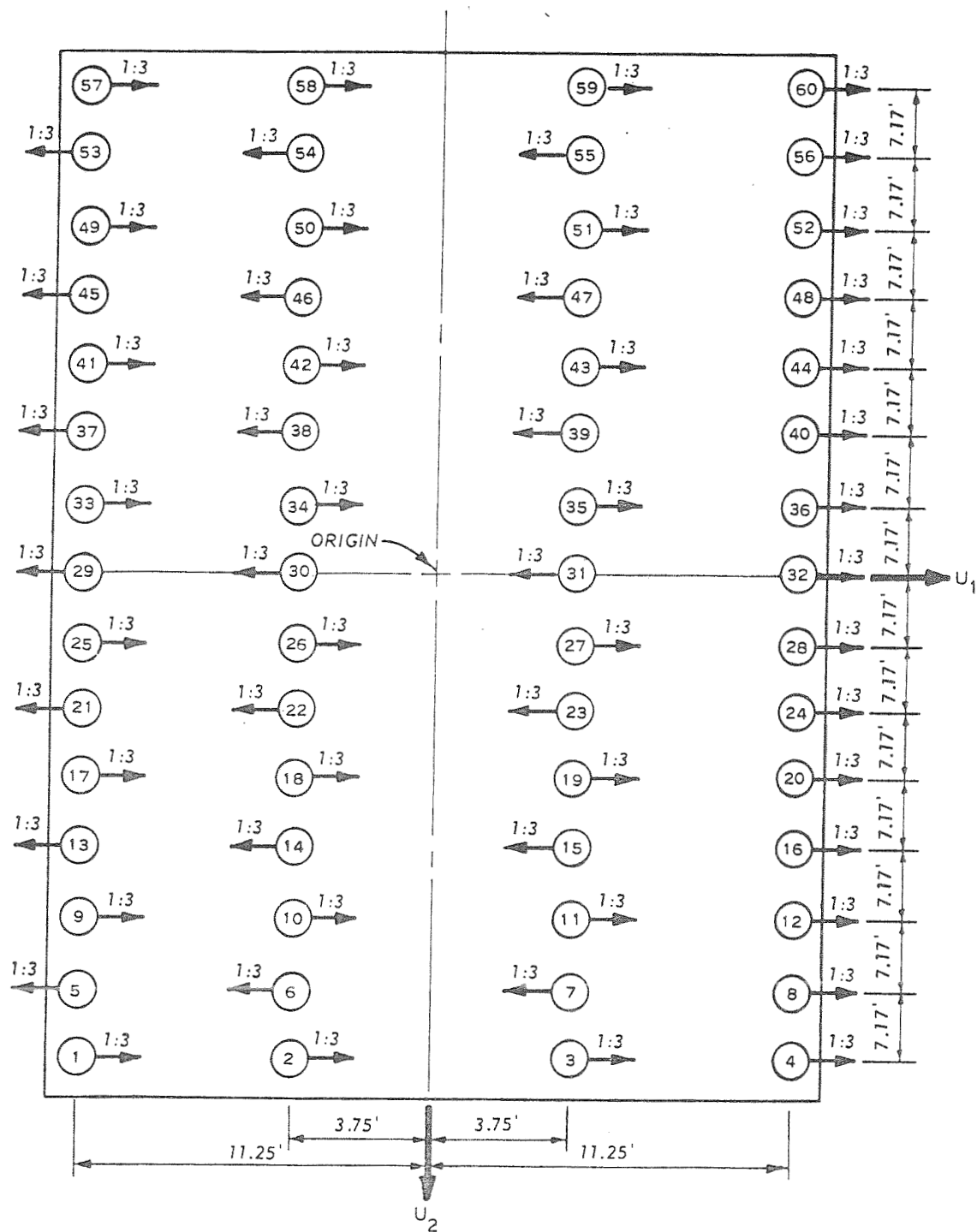
Figure 26. Physical problem for example problem 11
