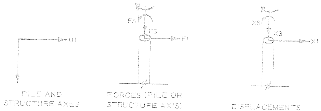
Figure 2. Coordinate system for two-dimensional system
