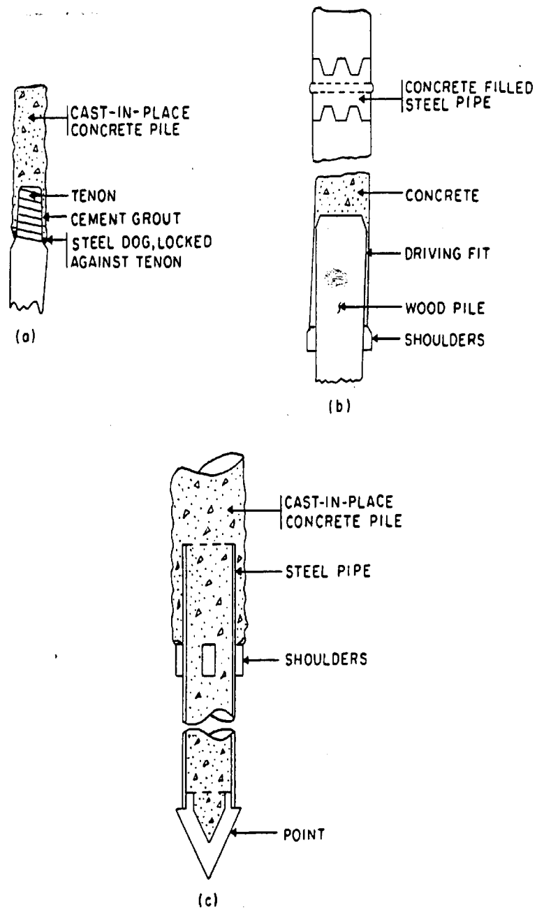
C. TYPICAL SPLICES FOR COMPOSITE PILES
