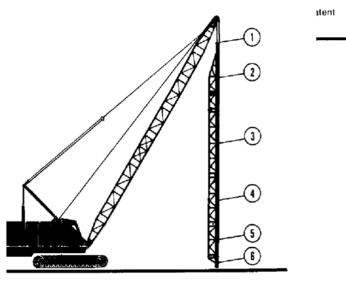
Figure 3-27. Vertical travel leaders.
