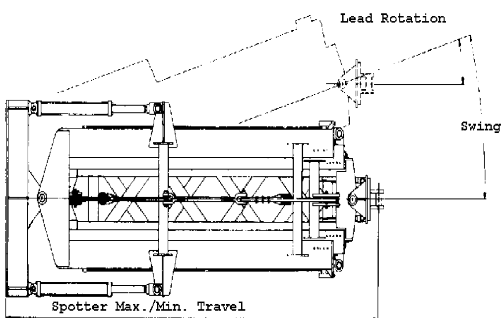
Figure 3-25. Moonbeam spotter leader.
