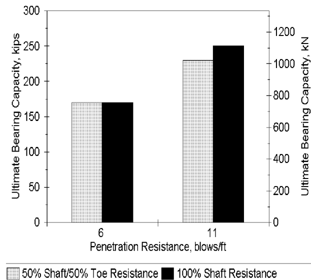
Figure 5-6. Wave equation analysis results.
