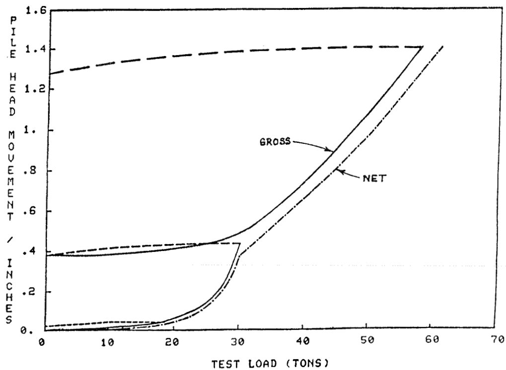
Figure B2. Test Pile 1, tension
