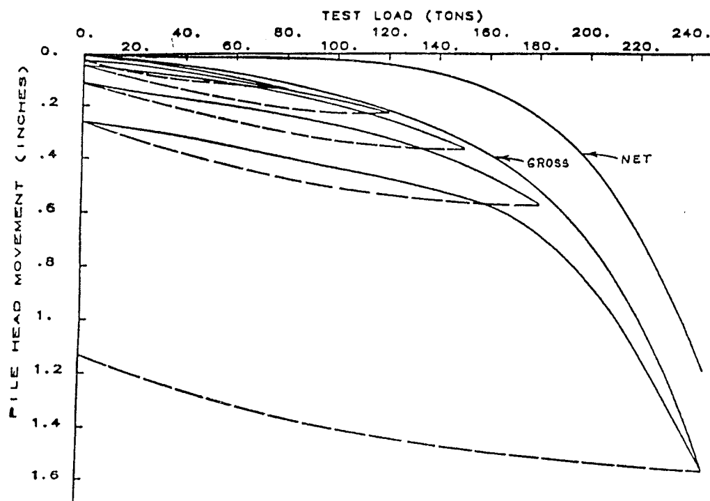
Figure B8. Test Pile 6, compression
