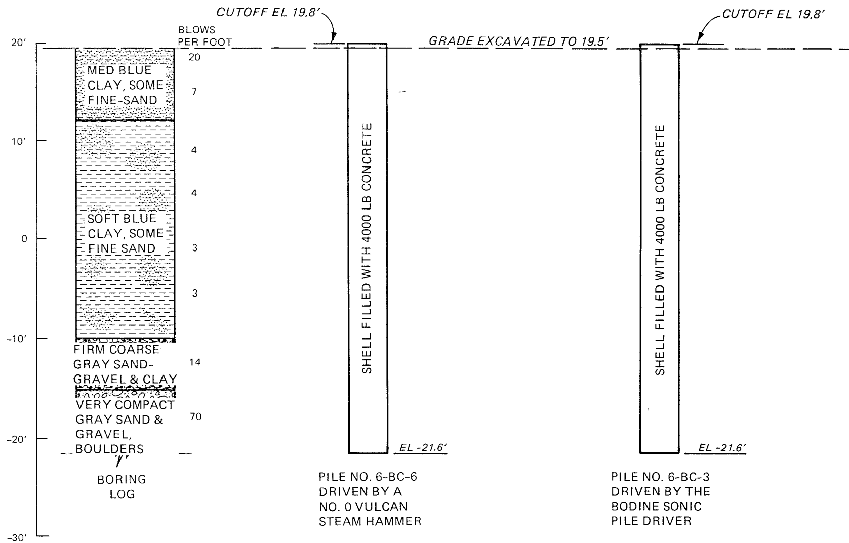
Figure 13. Soil profile for the Geochemical Building site
