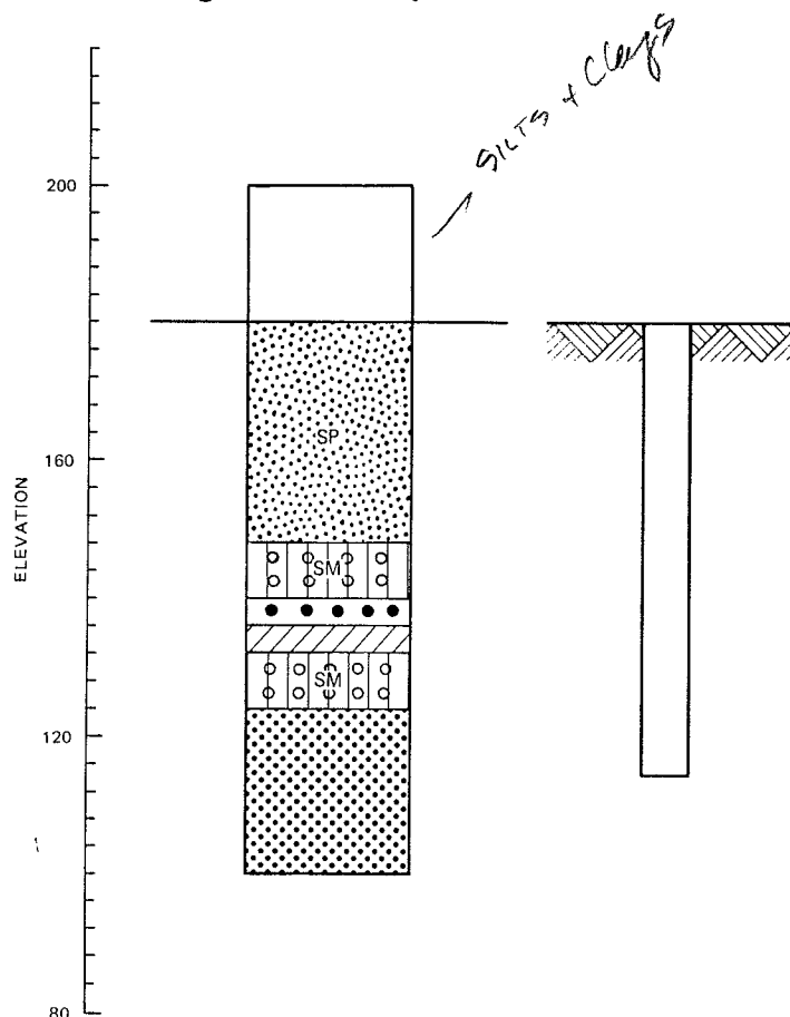
Figure 2. Generalized soil profile for Lock and Dam No. 4 pile test site
