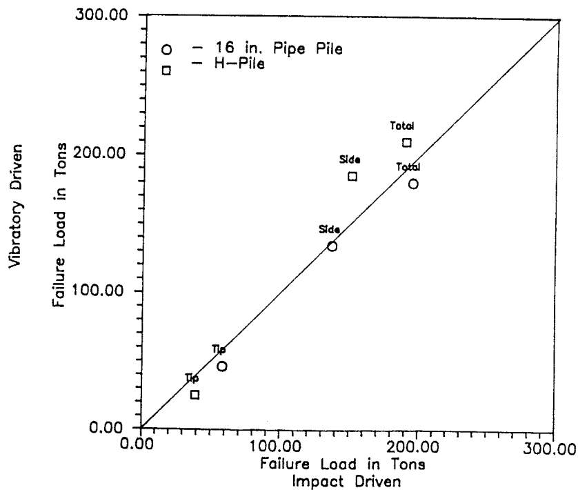
Figure 18. Comparison of load distribution of impact- and vibratory-driven piles for Lock and Dam No. 4
