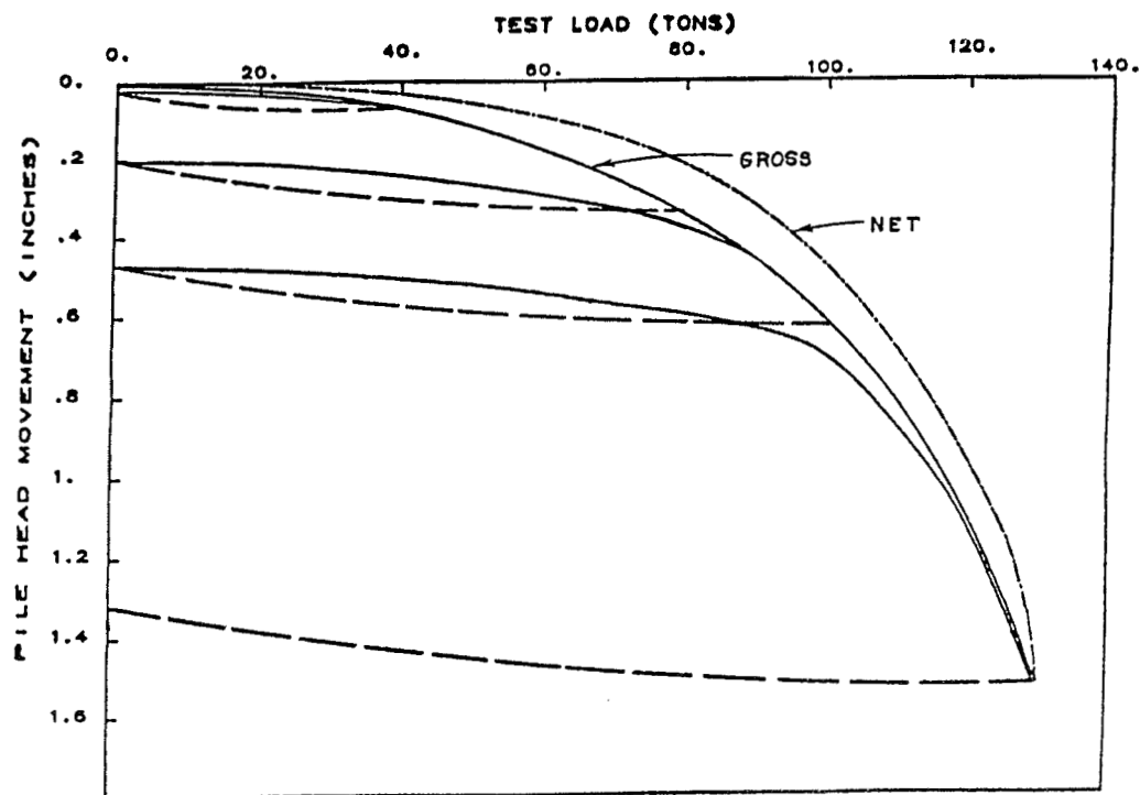
Figure B1. Test Pile 1, compression
