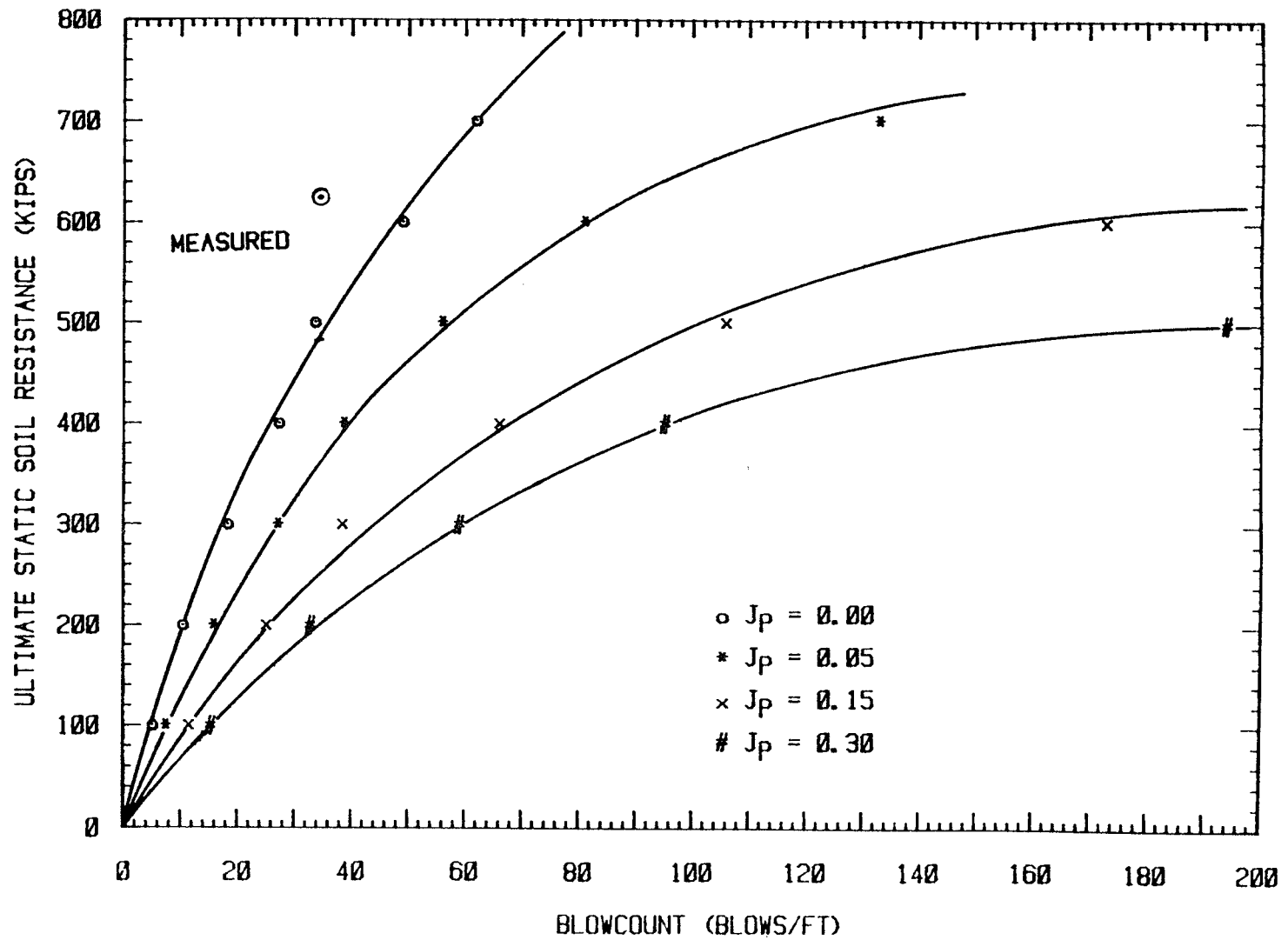
FIG. 28. RUT Versus N for Pile 1-3A Using 25% Secant Quakes
