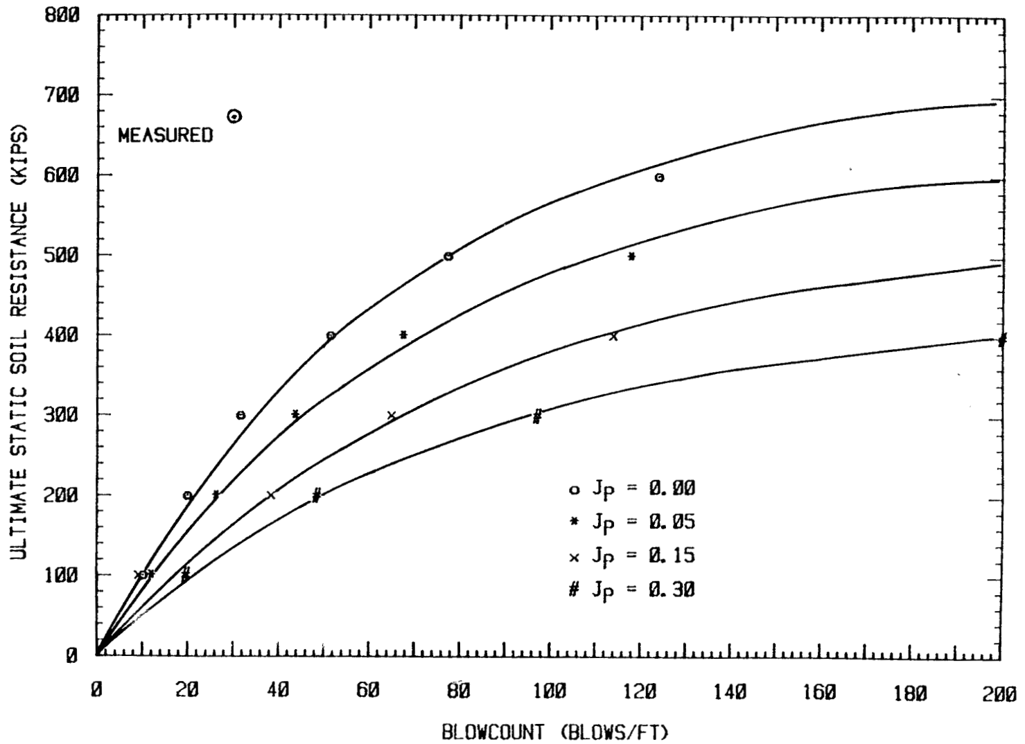
FIG. 29. RUT Versus N for Pile 1-9 Using 25% Secant Quakes
