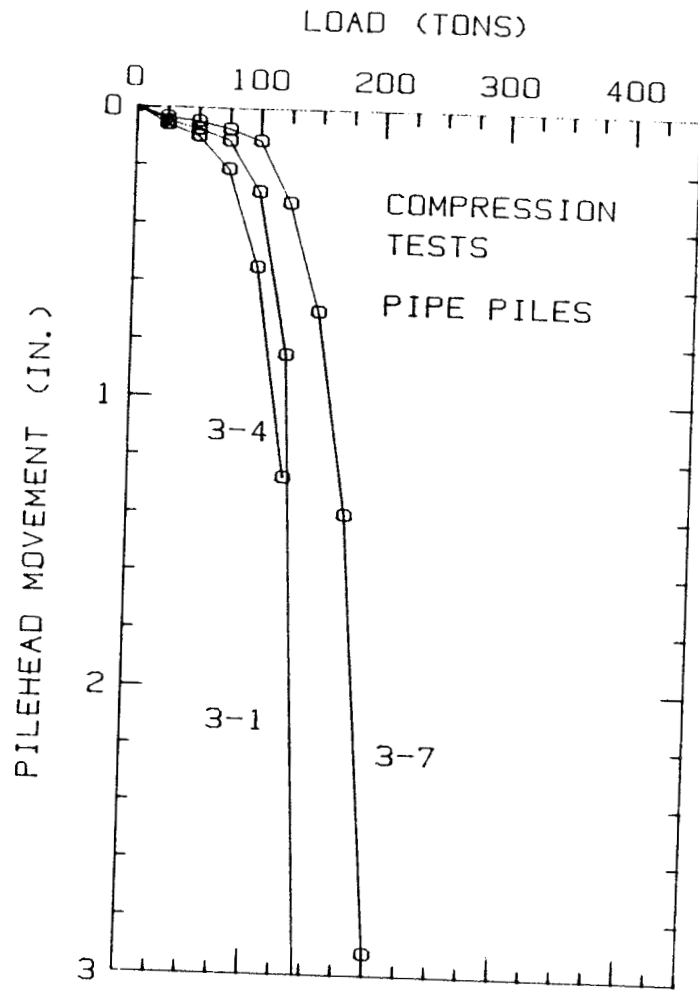
FIG. 19. Load Test Results for Compression Tests on Pipe Piles
