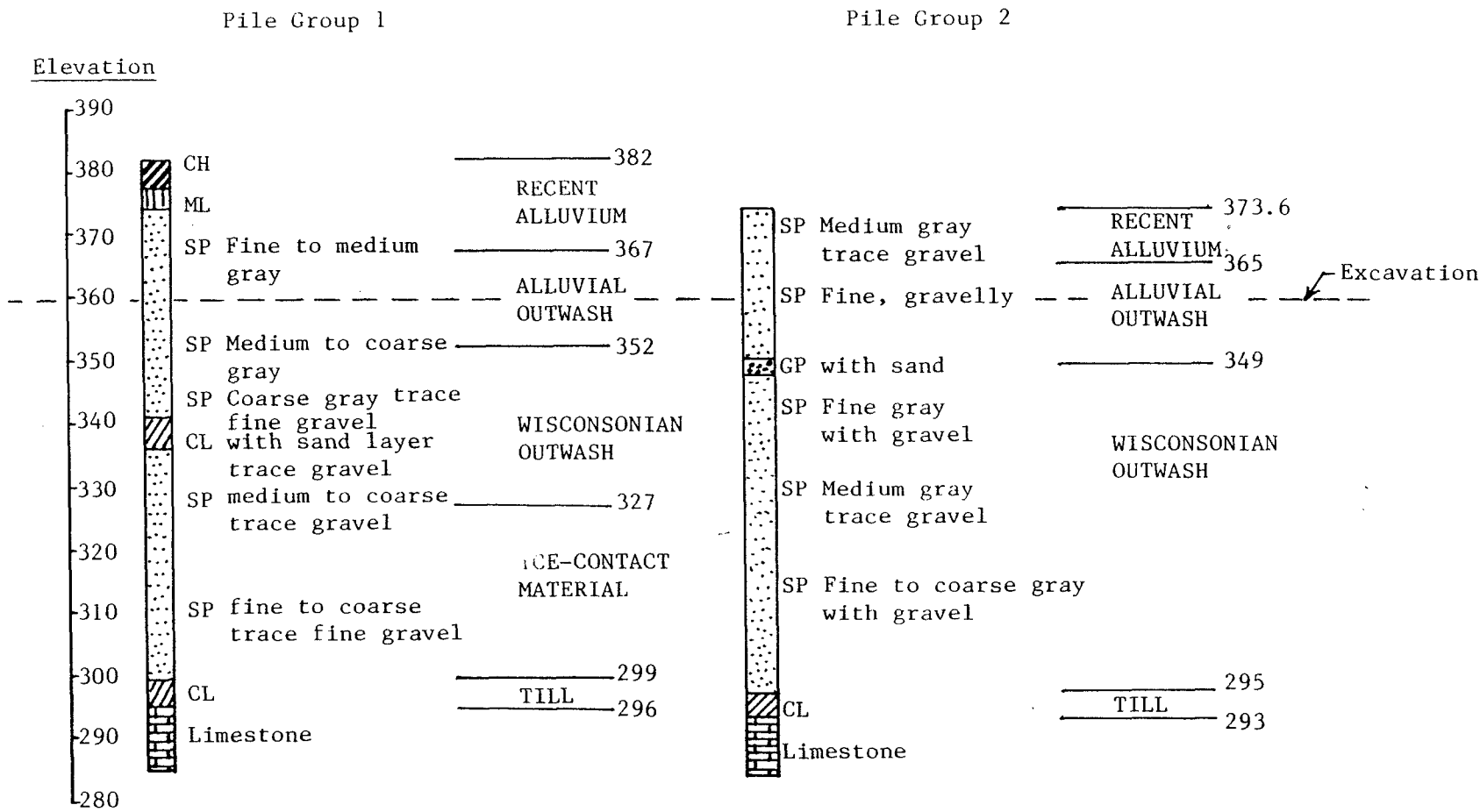
FIG. 3. Soil Profile Across Test Site
