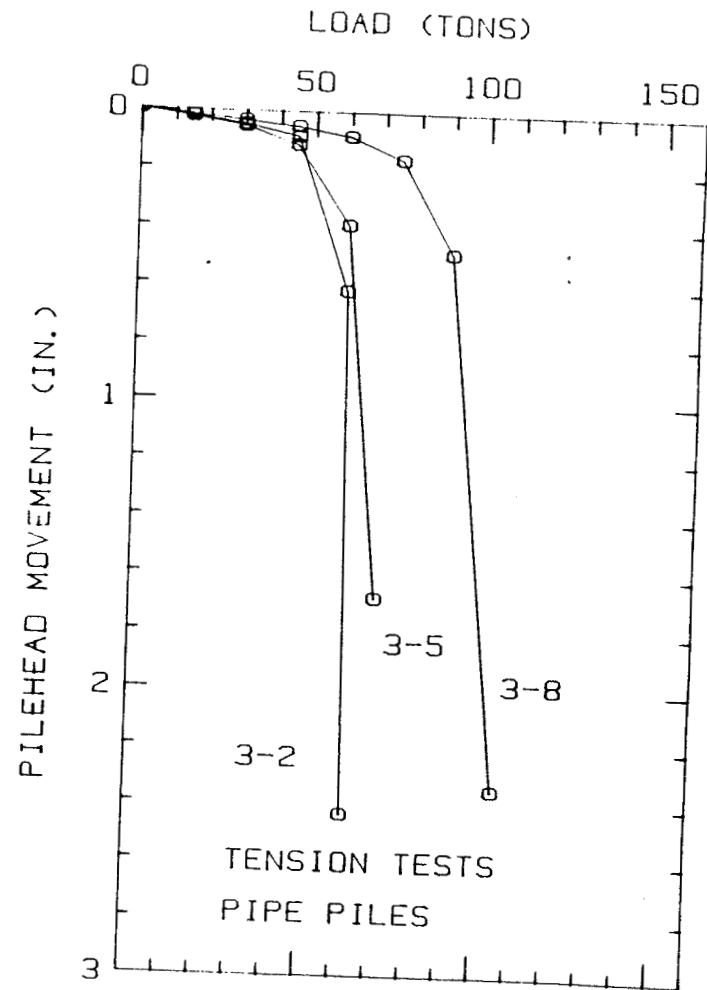
FIG. 20 Load Test Results for Tension Tests on Pipe Piles
