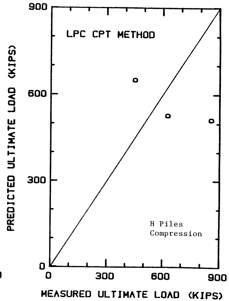
(b) Best CPT Method
