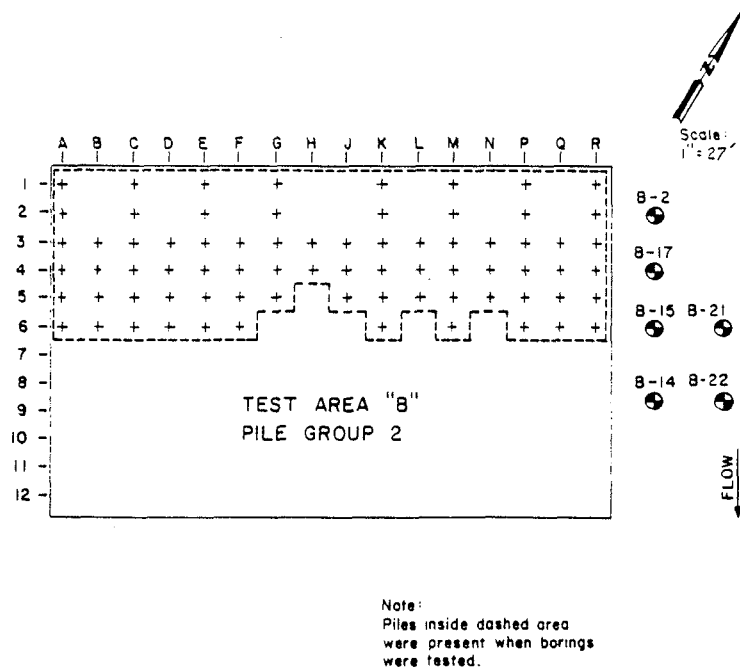
FIG. 6. In Situ Tests Borings for Pile Group 2
