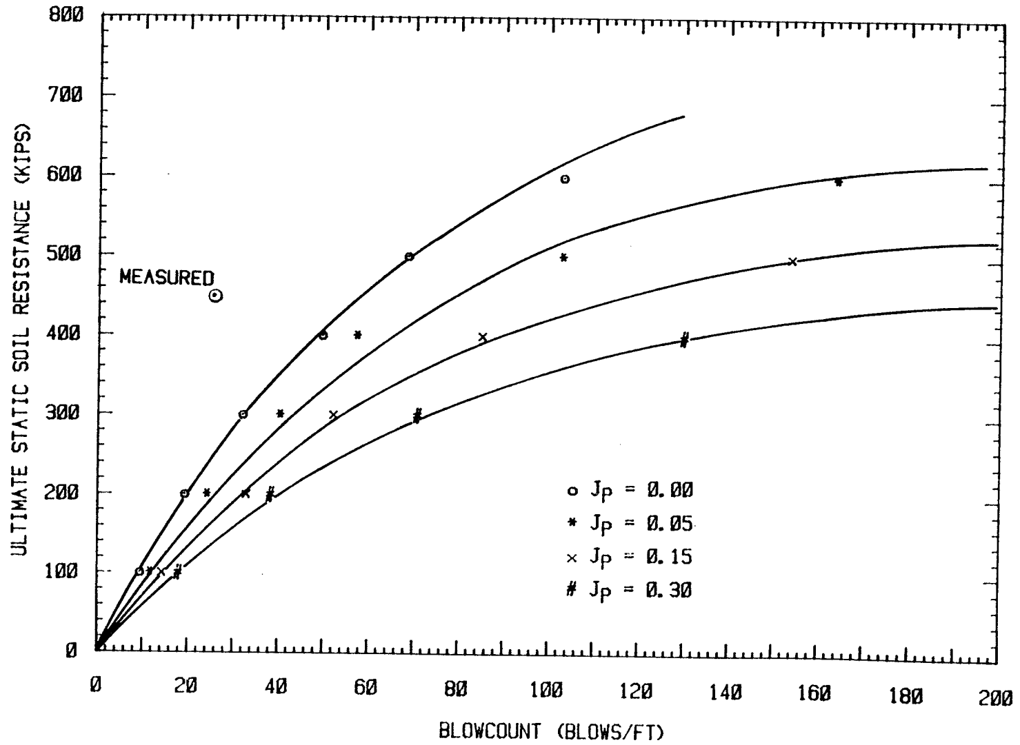
FIG. 30. RUT Versus N for Pile 2-5 Using 25% Secant Quakes
