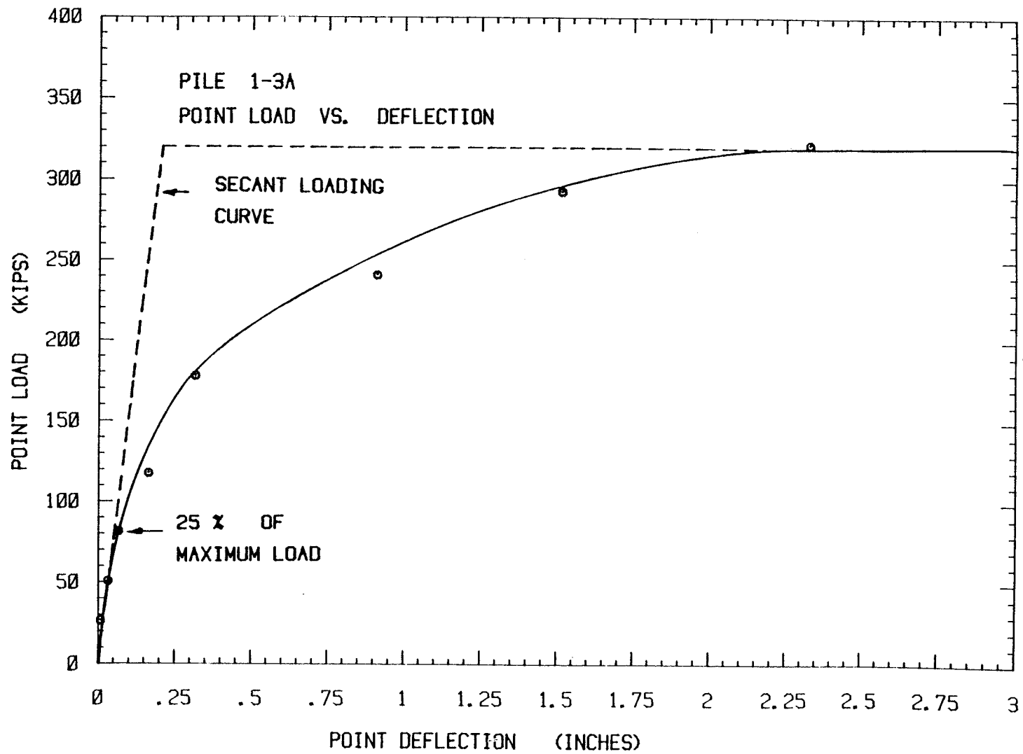
FIG. 27. Determination of 25% Secant Quake Values
