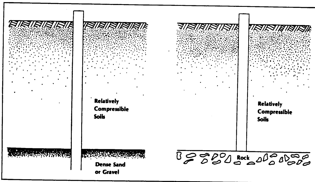
Figure 1-5 End-bearing piles
