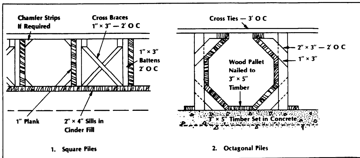
Figure 2-5 Wooden forms for casting concrete piles
