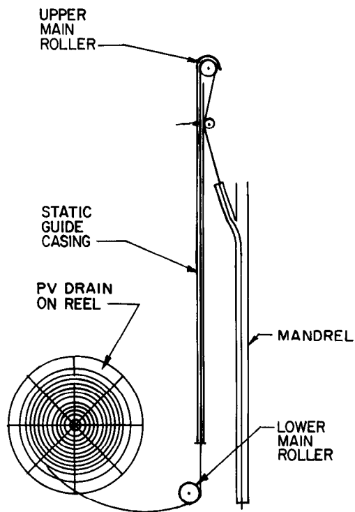
(B) DRAIN DELIVERY ARRANGEMENT
