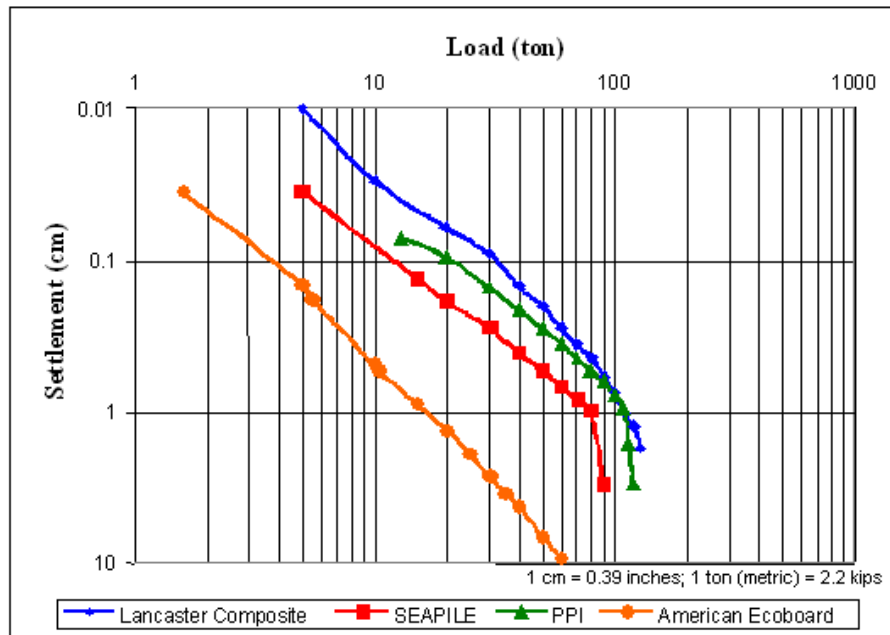
Figure 56. Graph. DeBeer criterion plotted for FRP piles.
