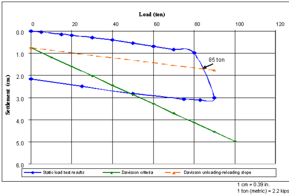
Figure 54. Graph. SEAPILE pile—Davisson criteria and measured load-settlement curve.
