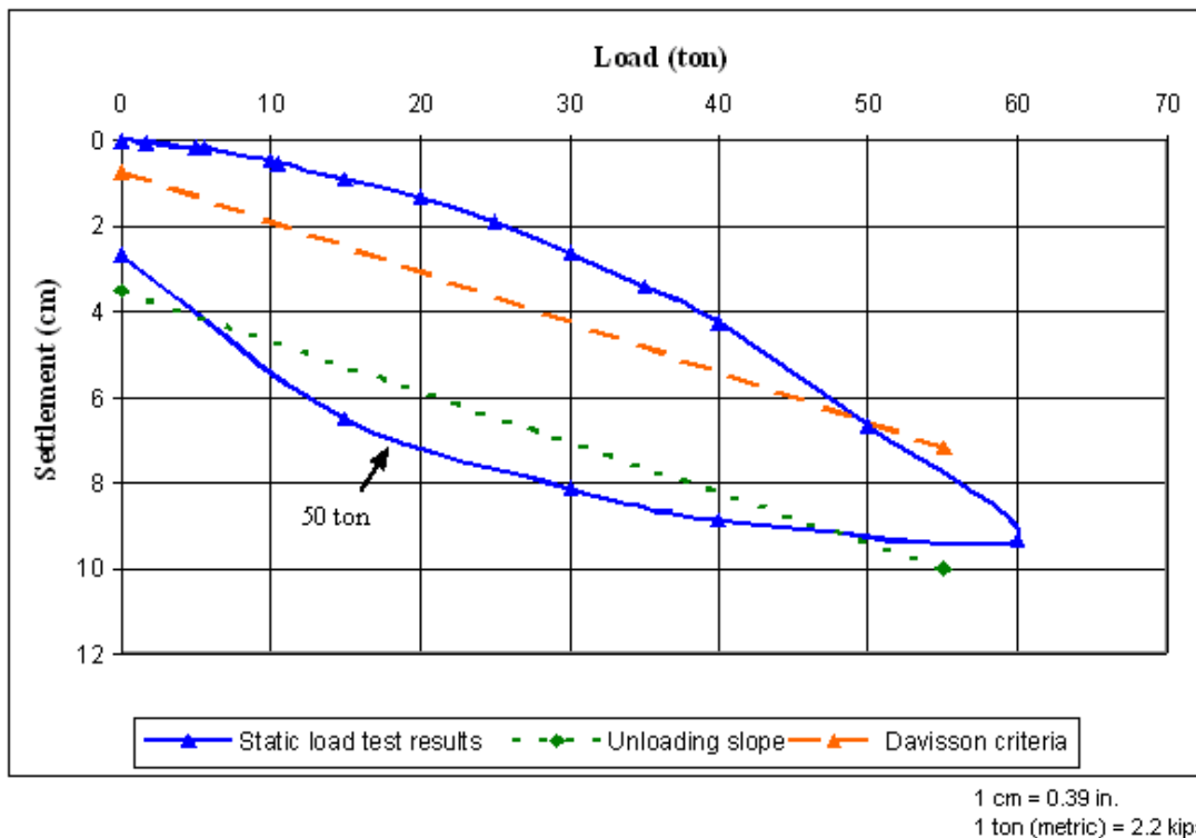
Figure 55. Graph. American Ecoboard pile—Davisson criteria and measured load-settlement curve.
