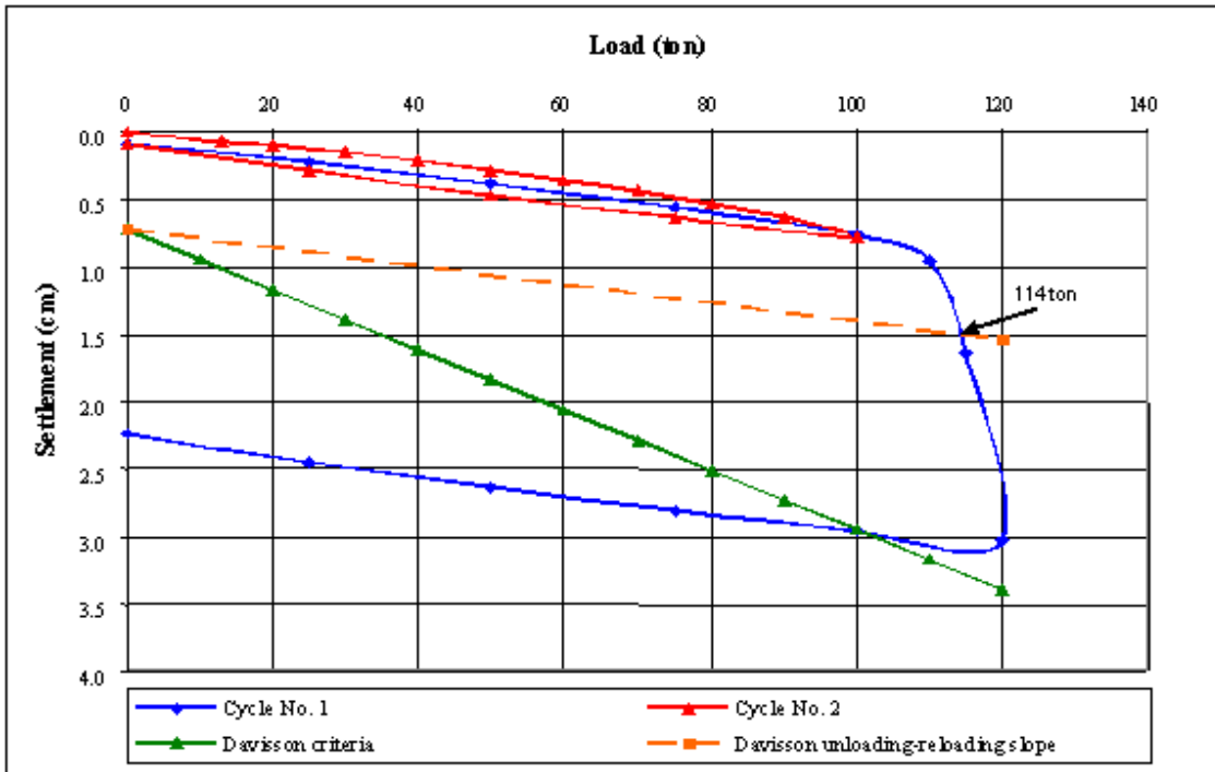
Figure 52. Graph. Lancaster Composite pile—Davisson criteria and measured load-settlement curve.
