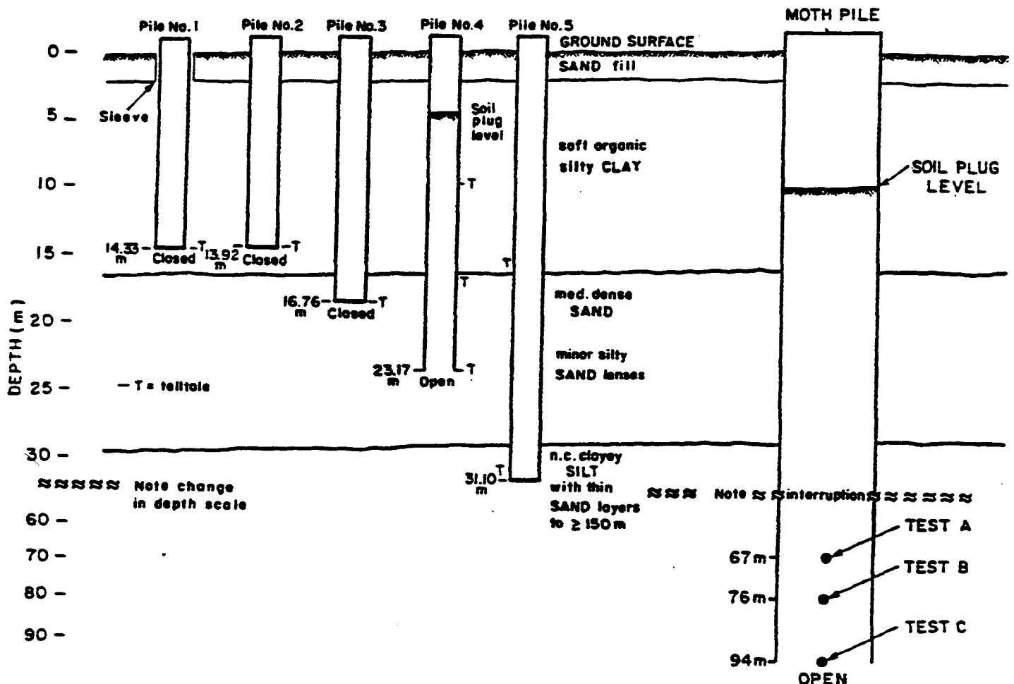
Fig. 3. Schematic of UBC/MOTH test pile embedments.
