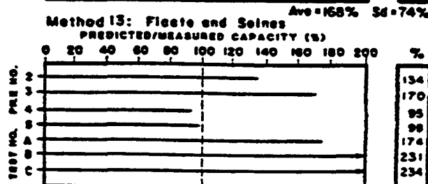
Fig. 8. Summary of predicted vs. measured axial pile capacity.
