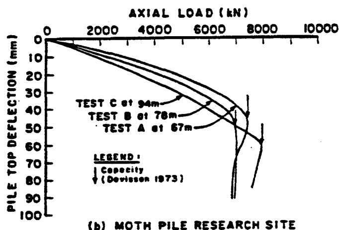
Fig. 5. Summary of axial load test results.
